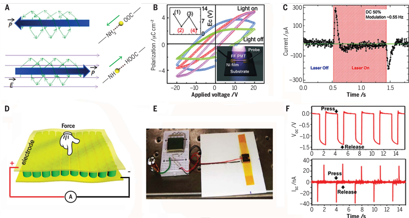
Fig. 5. Ferroelectric properties of FF self-assemblies. (A) Mechanism explaining the origin of spontaneous polarization and the predictable ferroelectricity of FF nanotubes. The short green arrows represent electric dipole moments of the hydrogen bonds; long blue arrows denote net electric polarization in the nanochannel. The spontaneous polarization in a nanotube is shown on the upper side, whereas the lower side shows that displacement of protons switches the spontaneous polarization under an alternative electric field (purple arrows). [Adapted from (77)] (B) Four polarization-electric curves obtained from the FF tubes during off/on switching of light. The inset shows
